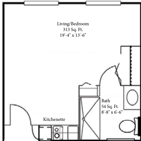
Studio A Floor Plan 400 Total Sq. Ft.
