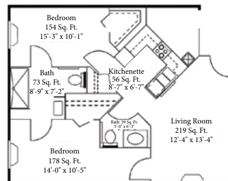
Two Bedroom Floor Plan 845 Total Sq. Ft.
